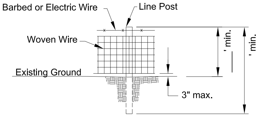
WOVEN WIRE WITH ONE BARB DETAIL
