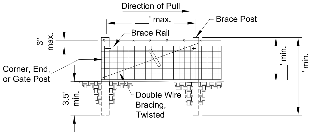
SINGLE SPAN BRACE ASSEMBLY (At Corners, Ends, or Gates)
