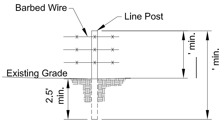
BARBED WIRE DETAIL
