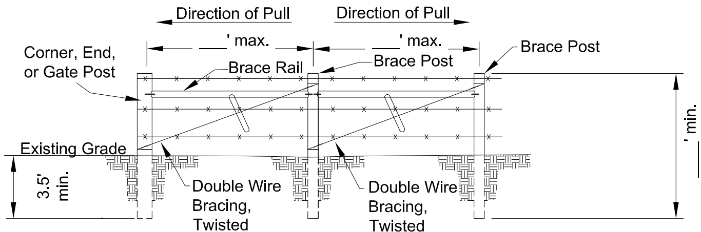
DOUBLE SPAN BRACE ASSEMBLY (at Corners, Ends, or Gates)
