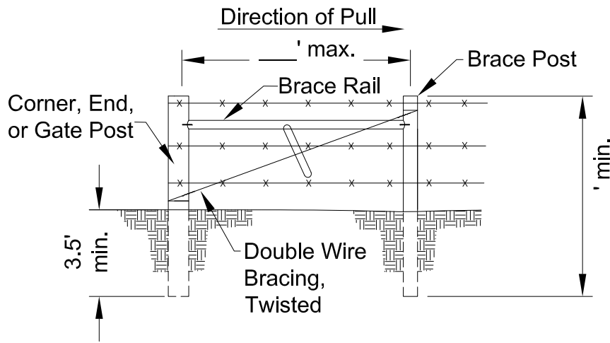
SINGLE SPAN BRACE ASSEMBLY (at Corners, Ends, or Gates)
