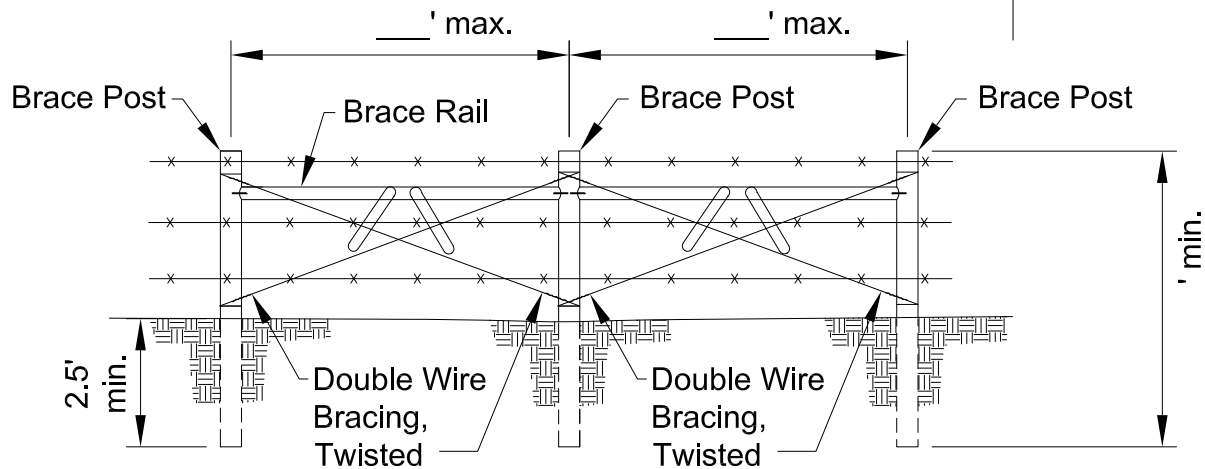
DOUBLE SPAN LINE BRACE ASSEMBLY
