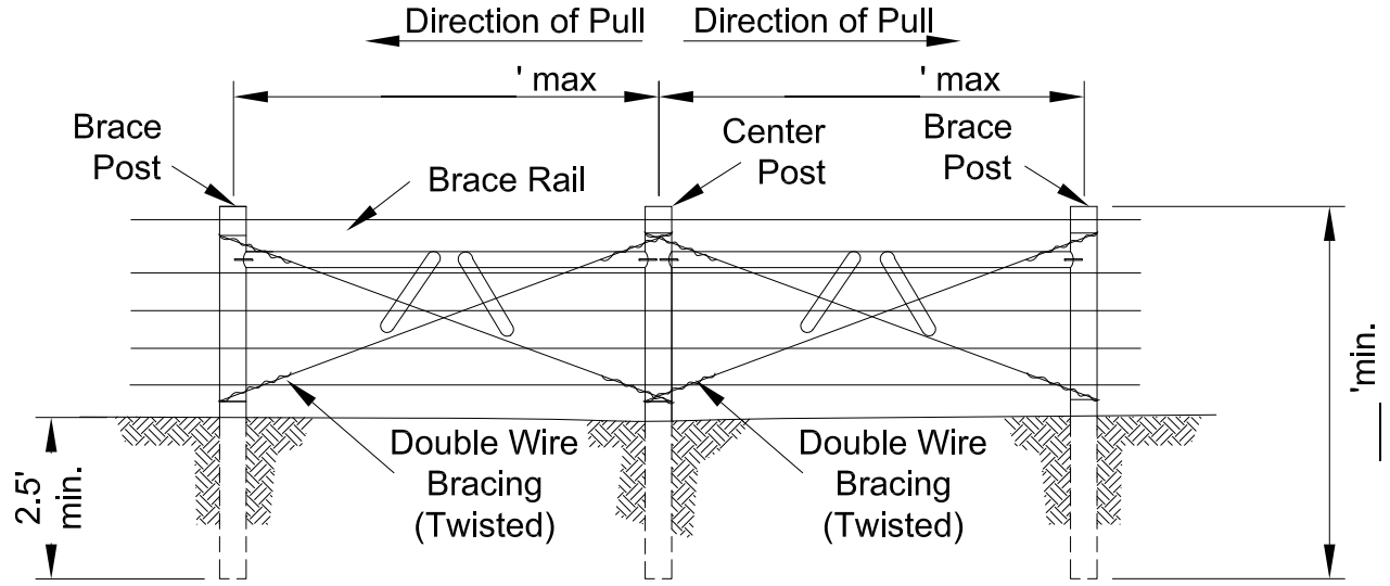
DOUBLE SPAN LINE BRACE ASSEMBLY
